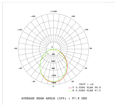
Courbe 50W - 2200K
