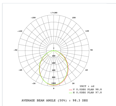
Courbe 30W - 2200K
