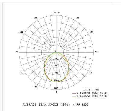
Courbe 20W - 3000K
