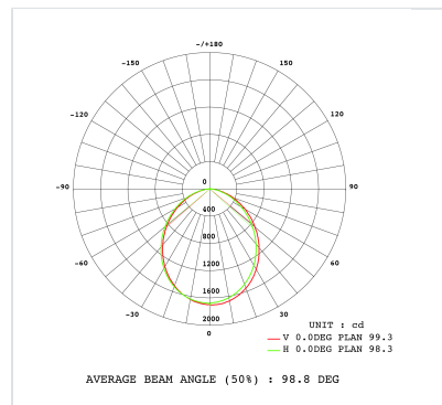
Courbe 50W - 4000K
