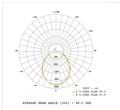
Courbe 50W - 3000K
