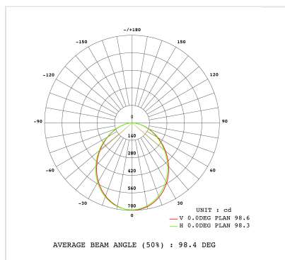
Courbe 20W - 2200K
