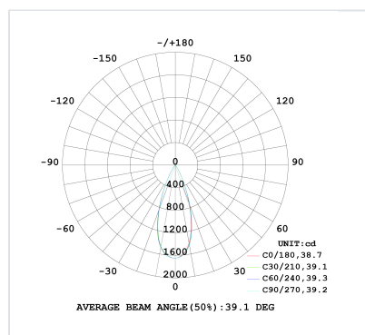
Courbe 11W 3000K
