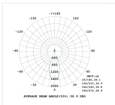
Courbe 11W 2700K
