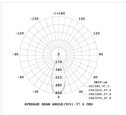
Courbe 6W 2700K
