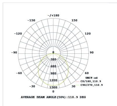
Courbe 36W - 3200K
