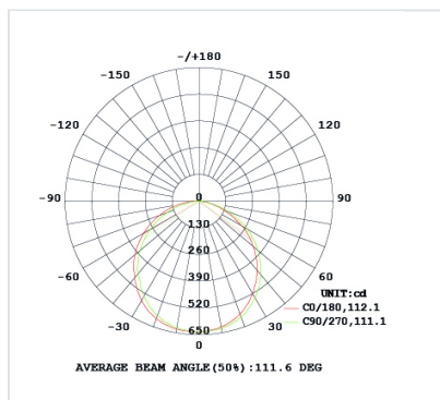
Courbe 20W - 2700K
