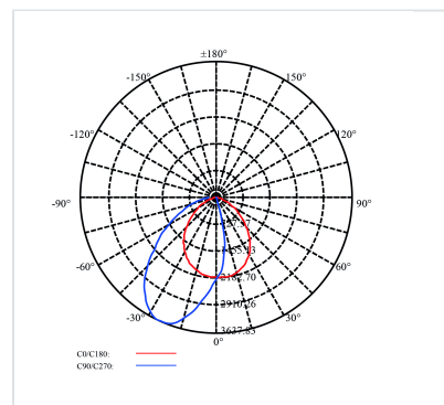
50W - 3000K+4000K-3500K
